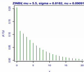
Zero inflated negative binomial type I, ZINBI
