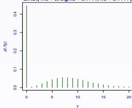
Zero inflated negative binomial type I, ZINBI
