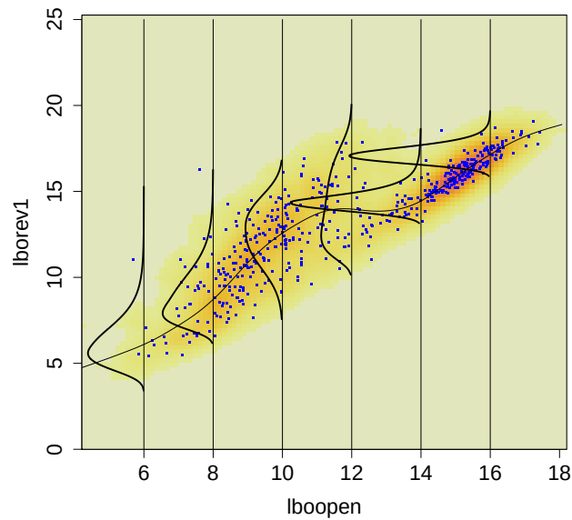
Figure 13: Fitted conditional distribution of the response variable lborev1 , showing how it changes for different values of the covariate lbopen .
